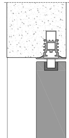
muratura - brickwall
