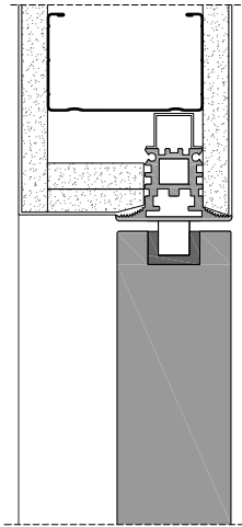
cartongesso - drywall
