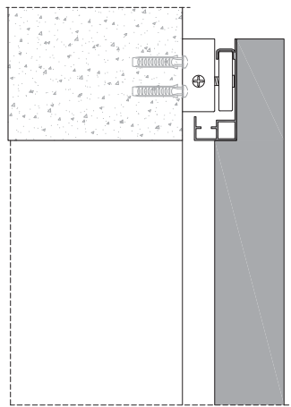
muratura ▪ brickwall
