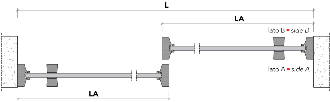
Schema traversini ■ Glazing bar position
