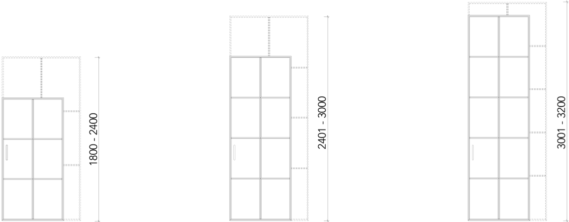
Schema traversini ■ Glazing bar position
