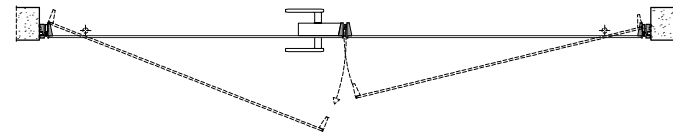
anta doppia a tirare double panel flush with pull side
