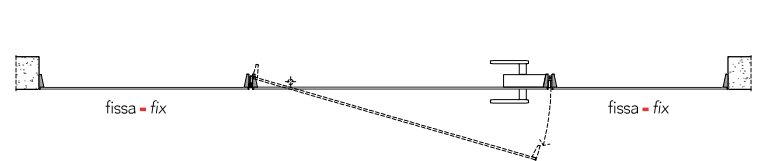
tre ante a tirare three panels flush with pull side
