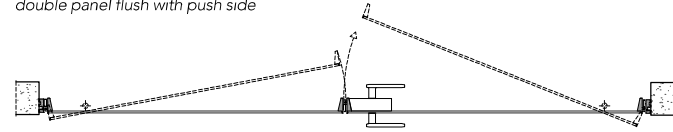
anta doppia a spingere double panel flush with push side
